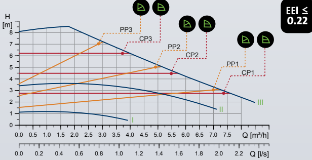
MAGNA1 25-80 (N)
