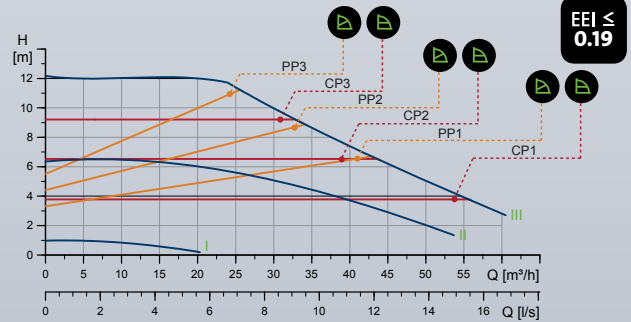
MAGNA1 80-120 F
